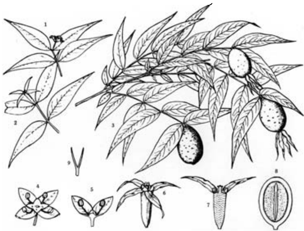
Buckleya distichophylla . 1. Flowering branch of the staminate plant, natural size. 2. Flowering branch of the pistillate plant, natural size. 3. Fruiting branch, natural size. 4. Staminate flower, enlarged. 5. Vertical section of a staminate flower, enlarged. 6. Pistillate flower, enlarged. 7. Vertical section of a pistillate flower, enlarged. 8. Vertical section of a seed, somewhat enlarged. 9. Embryo, much magnified. From Garden and Forest , 3:237. 1890.
